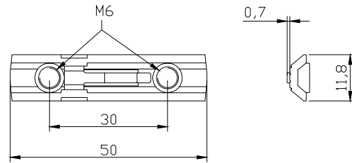
Figure 35 - Fastening inserts FI
