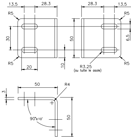
Figure 34 - Fastening brackets LL
